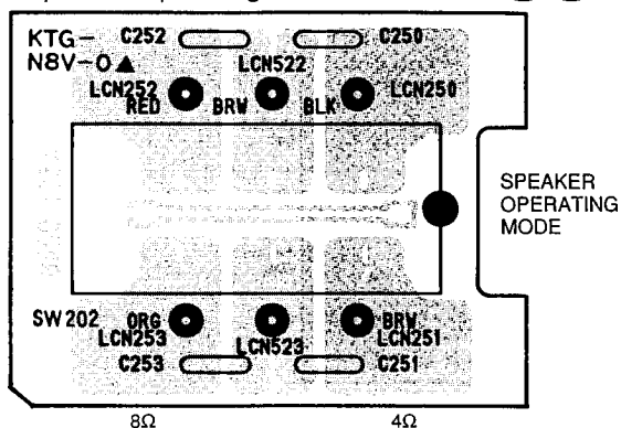
PCB-13 Speaker Operating Mode P. C. Board BK WB
