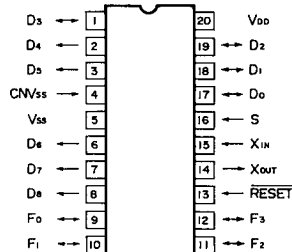
IC201 M50761-281P
