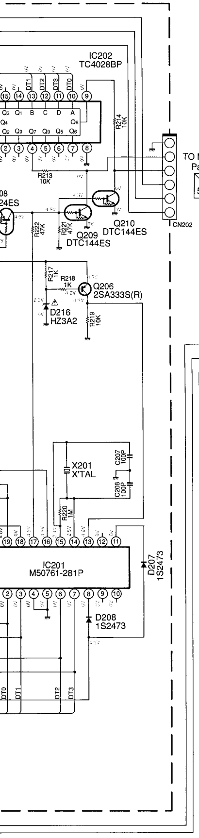
IC201 M50761-281P
