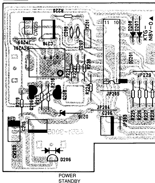
PCB-14 Remote P. C. Board
