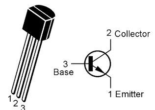
2SC1815 Q101,102,111,112,113,115,118,201, 206,207,208,301,302
