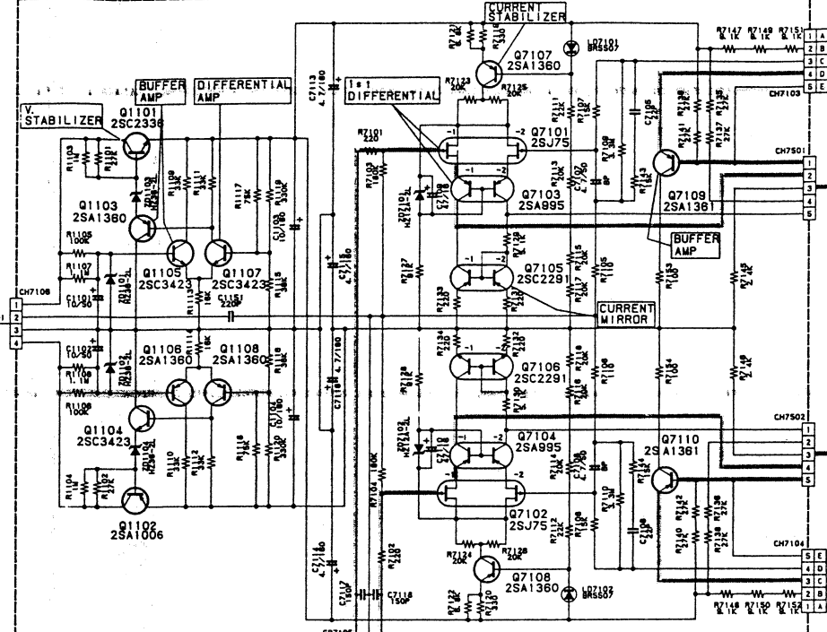
DRIVER P. C. Board
