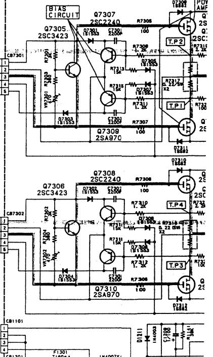
MAIN P. C. Board
