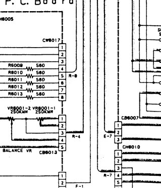
FUNCTION P. C. Board
